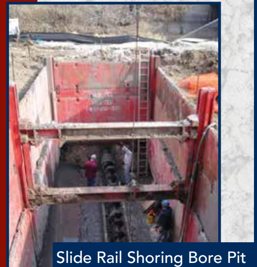
Vertical Hydraulic Shoring
